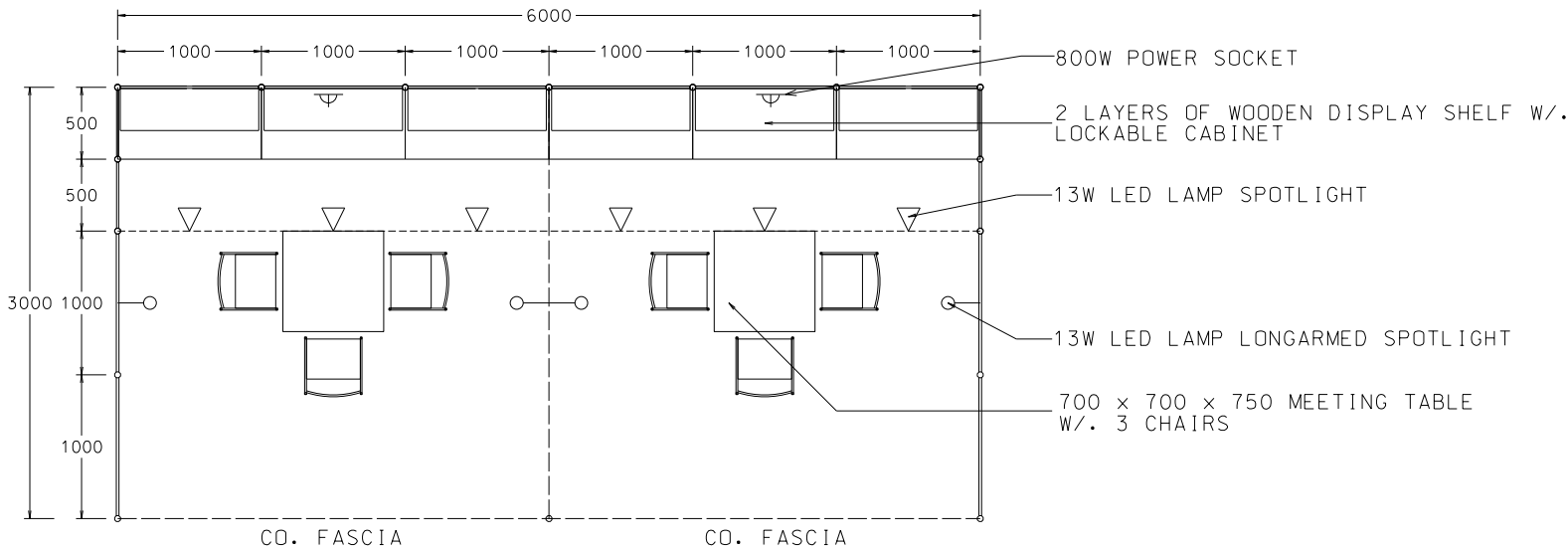
PLAN
