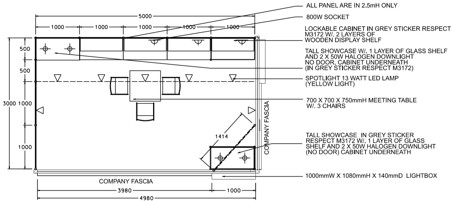
PLAN
